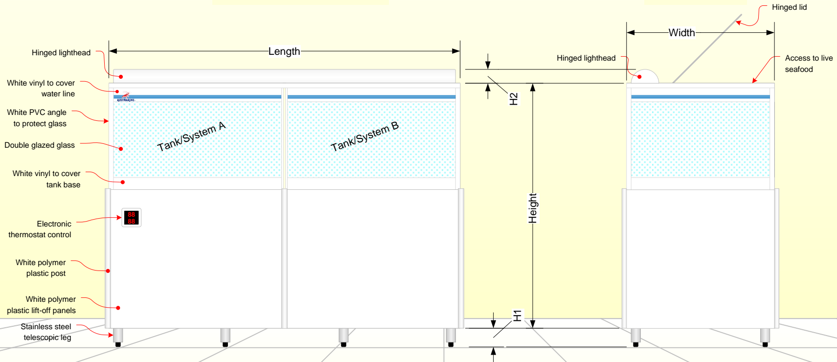
Front Elevation View – Access Side
