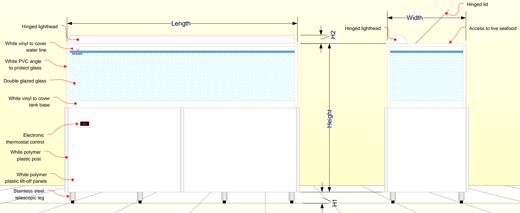
Front Elevation View – Access Side
