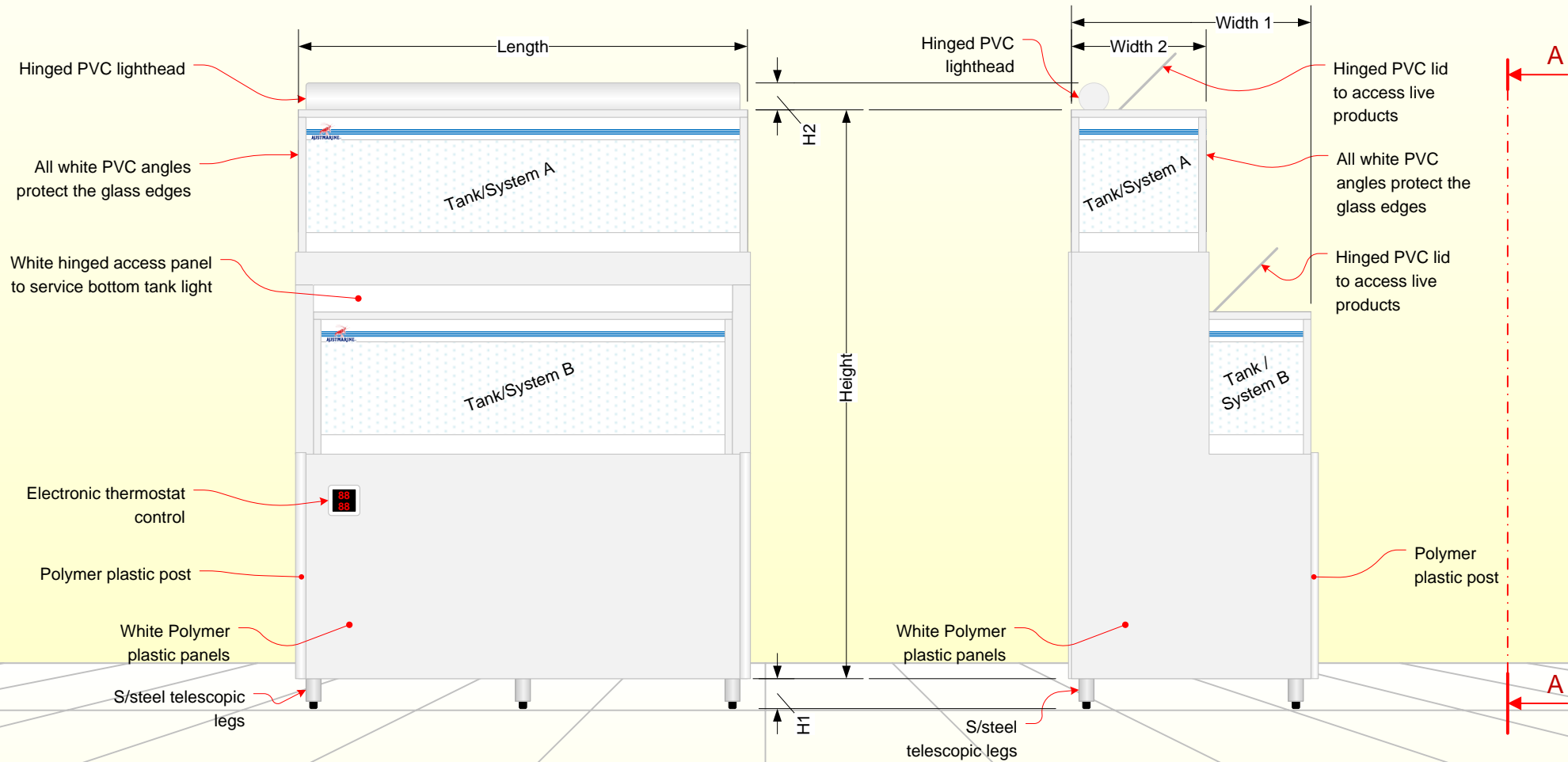
Access Side Elevation Section A:A View
